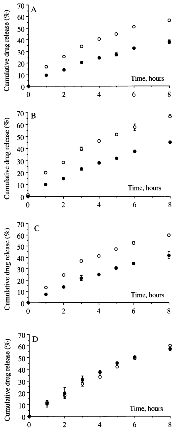
Fig. 4. The release kinetics of Scef (empty circles) and Ib (filled circles) from formulations A, B, C and D. Shown are the mean results of three tablets \pm S.D.
